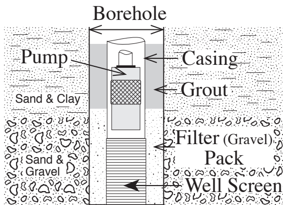
Filter Pack and Related Structures
